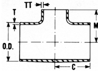
A7RW Reducing Tee
