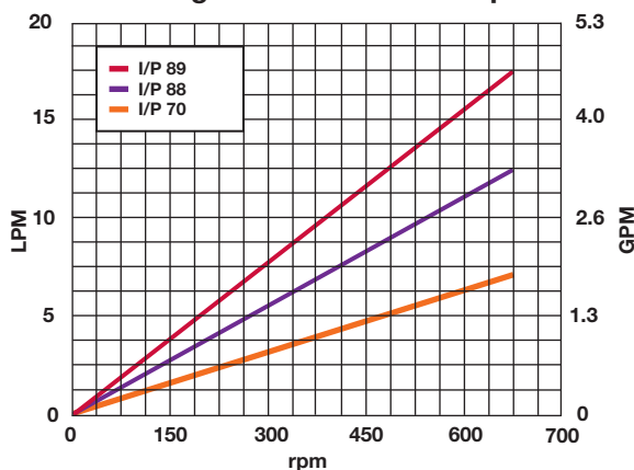
Flow Curves I/P High-Performance Pump
