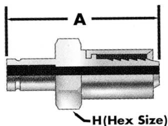
Tube Adapter with Nut & Ferrule Specifications Style 32FN
